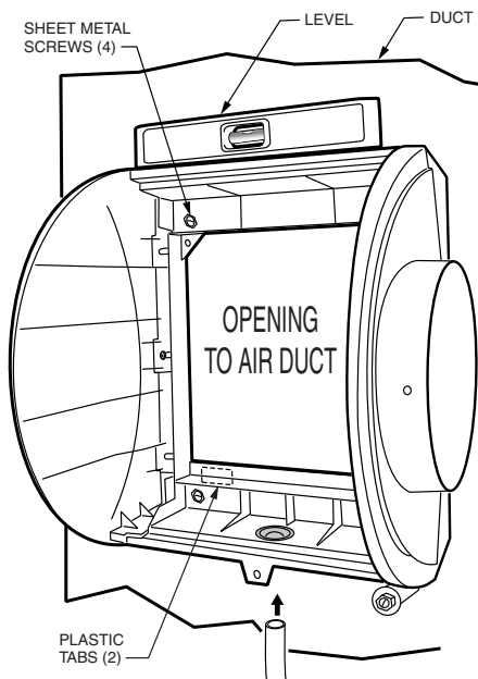
Fig. 4. Installing humidifier on duct.
