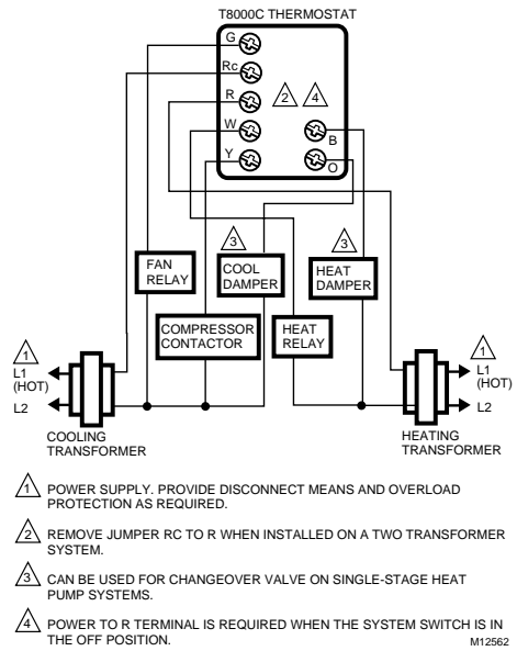
Fig. 6. Typical hookup of T8000C in heat-cool system with two transformers.
