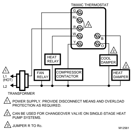
Fig. 5. Typical hookup of T8000C in heat-cool system with single transformer.
