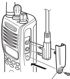
Speaker/ microphone locking bracket
