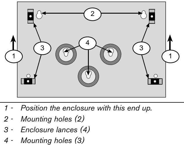
Figure 2: Mounting
