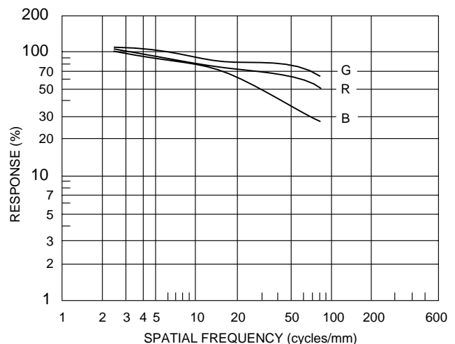
Modulation-Transfer Curves
