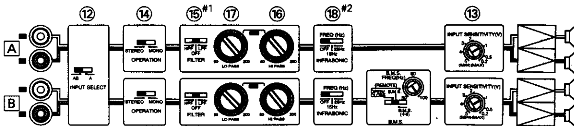
Block diagram
