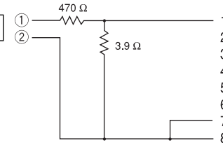
To 3.5 mm (1/8") speaker jack
