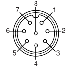
MIC connector on HF transceiver
