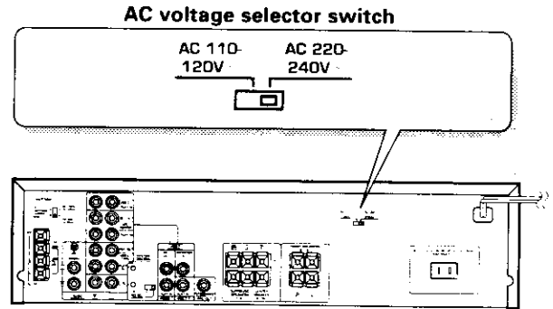
Move switch lever to match your line voltage with a small screwdriver or other pointed tool.
