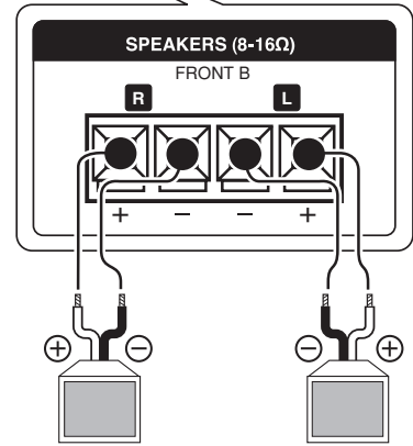
Front Speakers B
