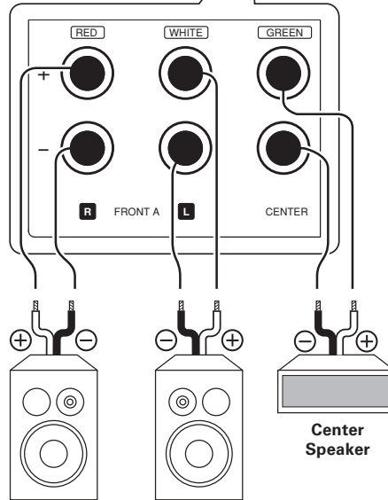
Front Speakers A
