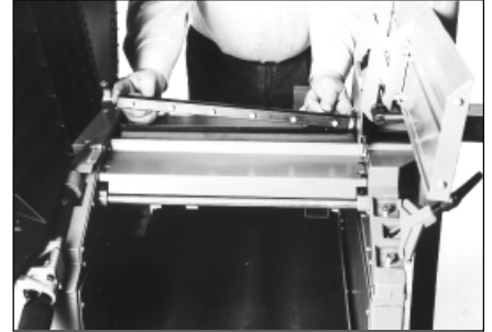
Max. planerblade projection over the cutterblock is 1.0 mm.
