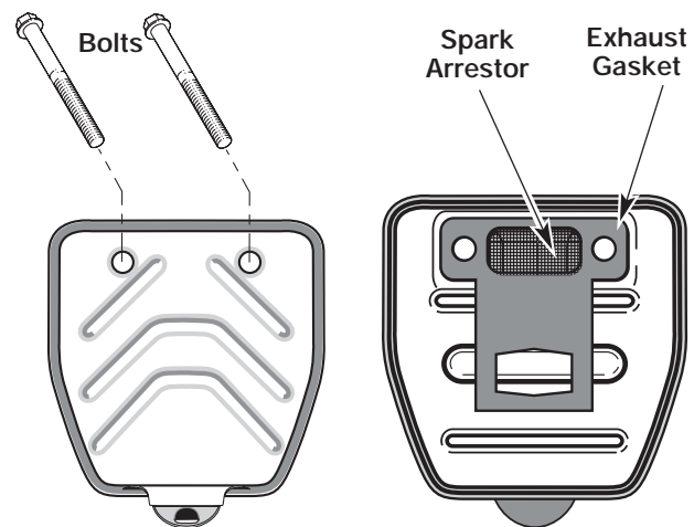
Muffler - Front Side
