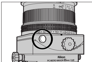
Stop-down aperture
