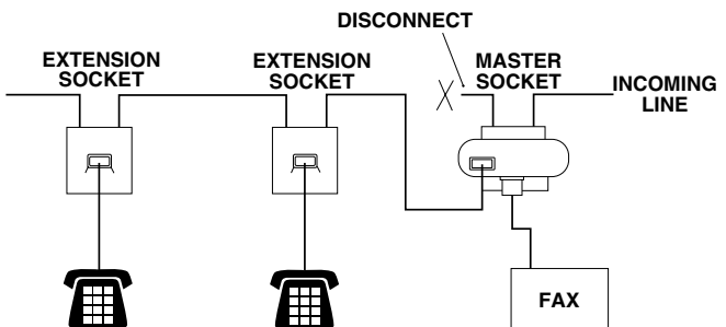
RECOMMENDED CONNECTION OF EXTENSION SOCKETS Fig. 2.
