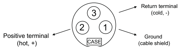
XLR Terminal (male) Pins on BDP-95
