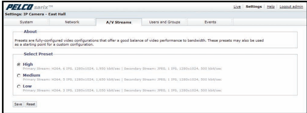
Figure 4. Select Video Preset Configuration Page
