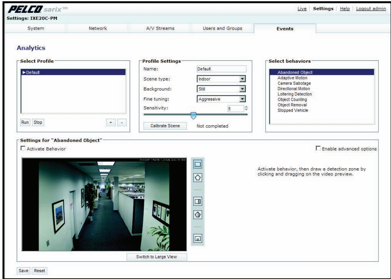
Figure 12. Analytic Configuration Page
