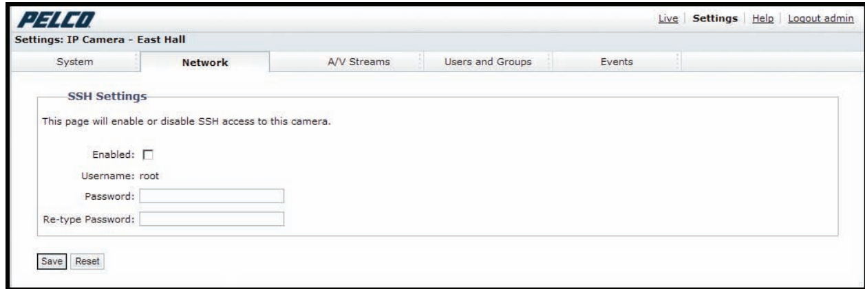
Figure 3. SSH Settings Page
