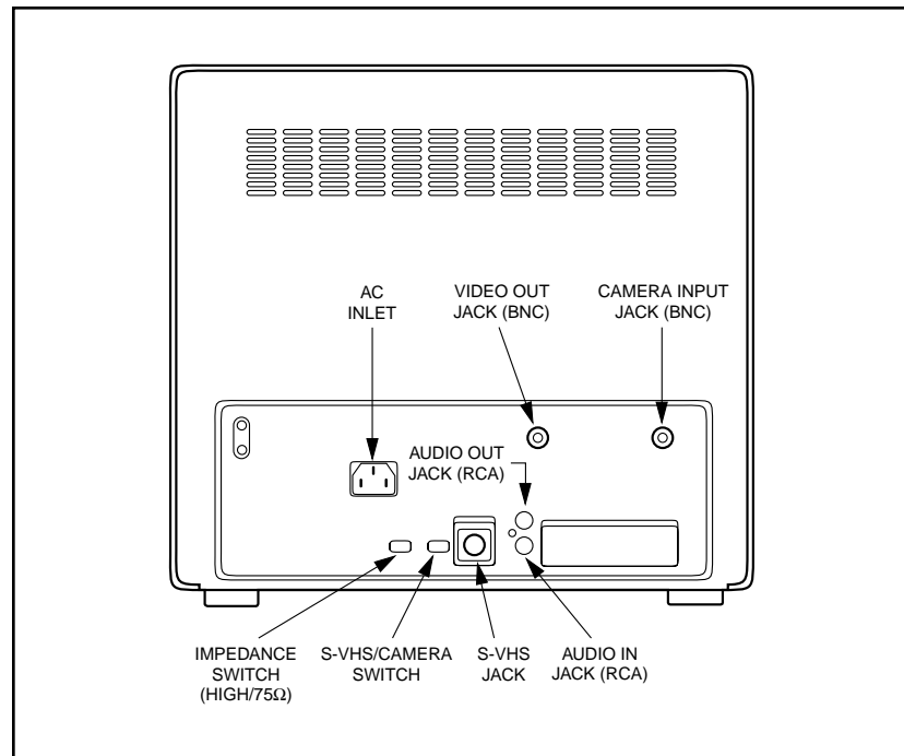
Figure 1. Rear Panel Connections
