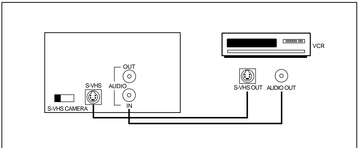
Figure 4. S-VHS Video (Y/C) Input Connections
