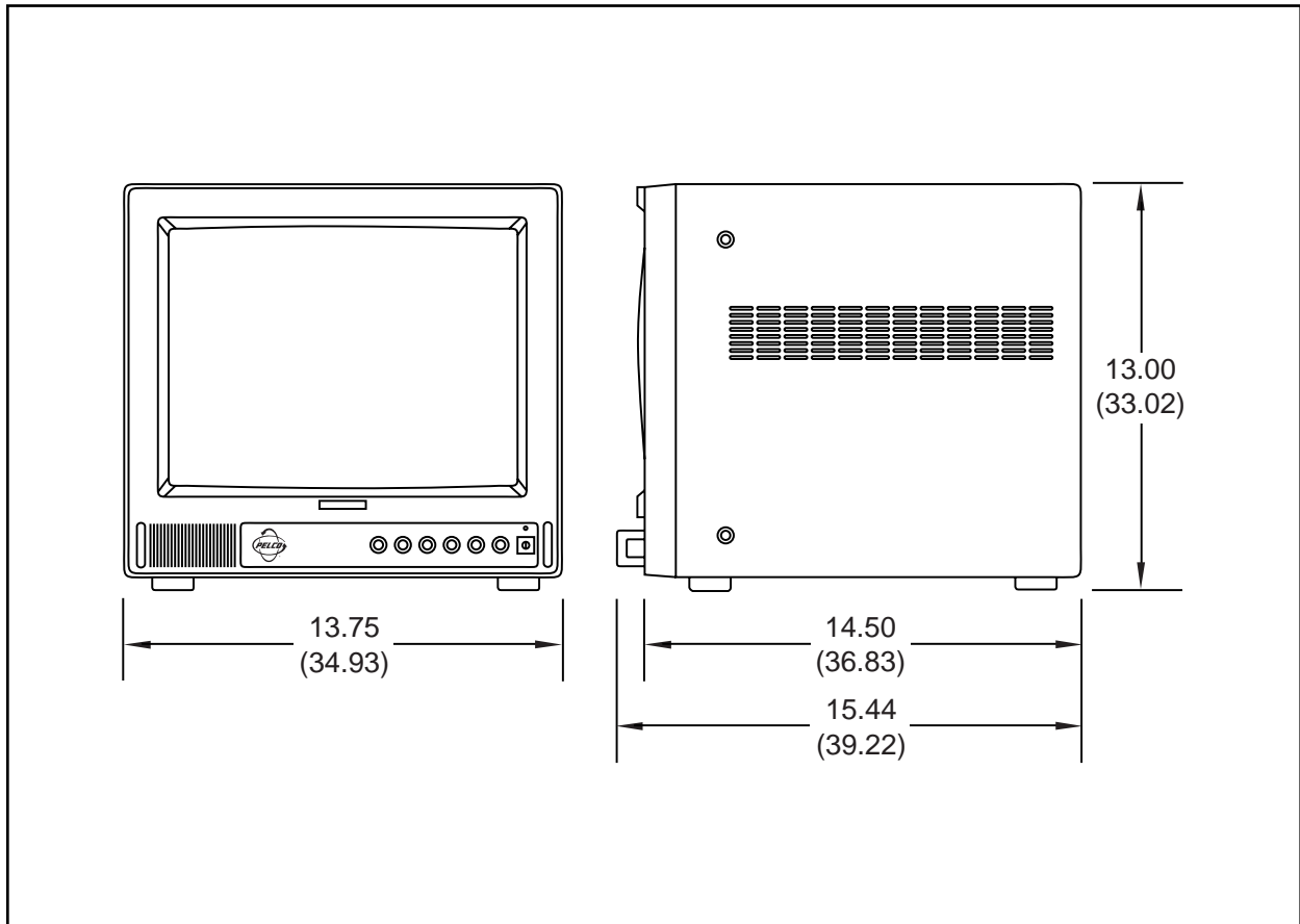
Figure 6. PMC14F Series Dimension Drawing
