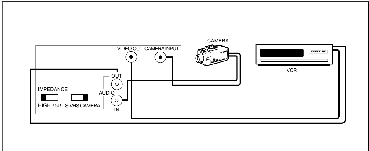
Figure 2. One Monitor with External Video Equipment
