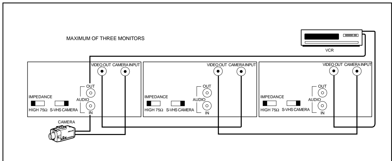
Figure 3. Monitor Looping with External Video Equipment
