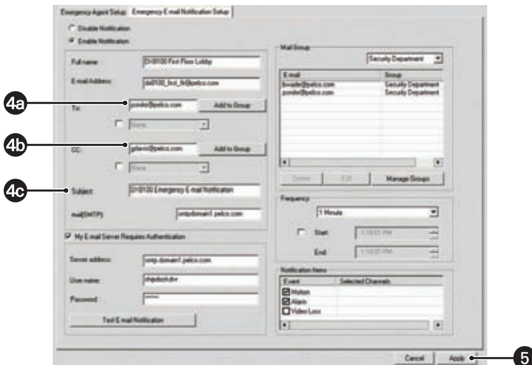
Figure 150. Sending E-mails to Individuals
