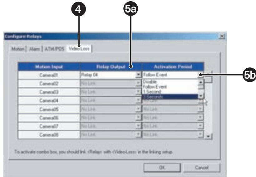
Figure 133. Linking Relays to Video Loss
