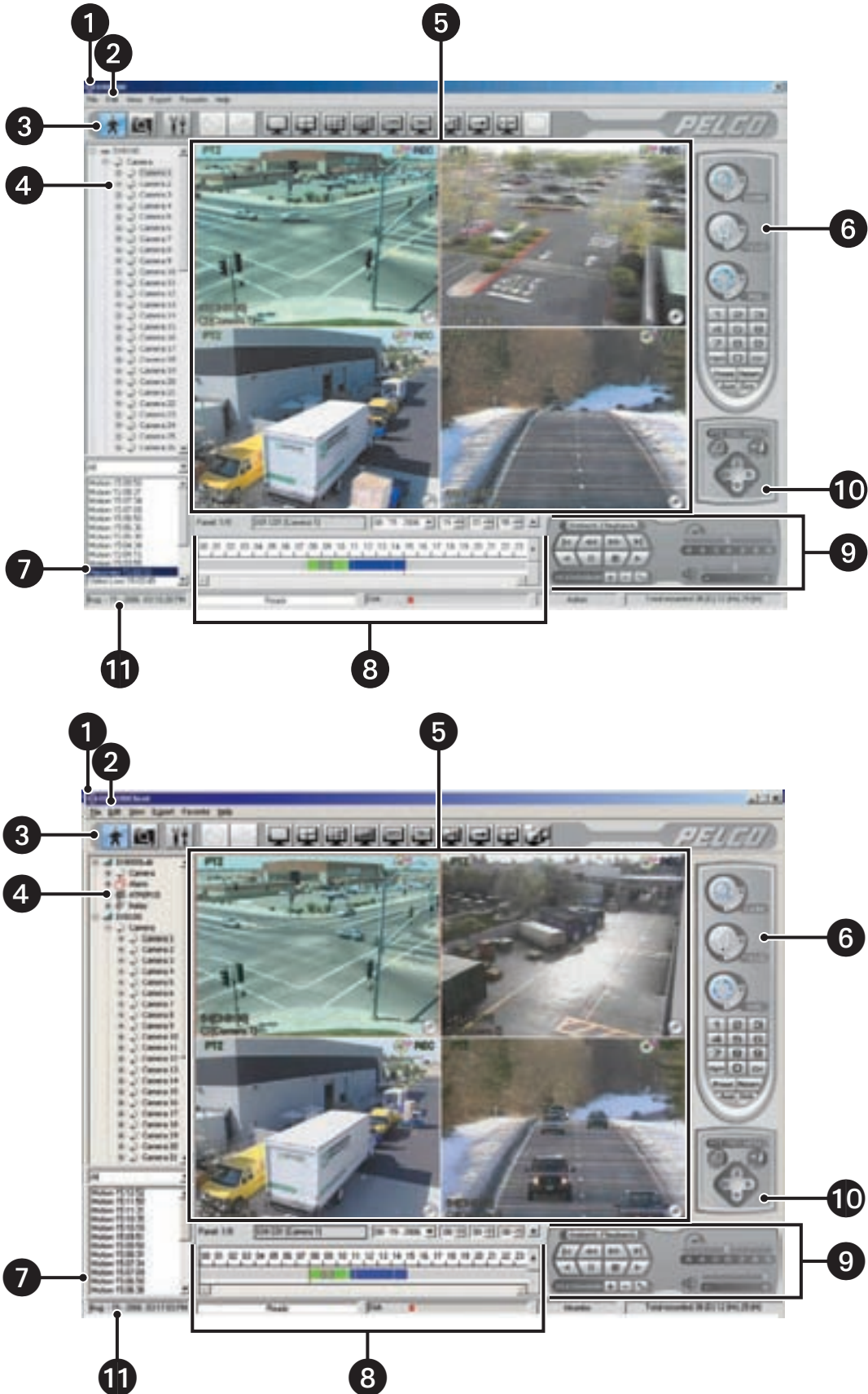
Figure 17. DX8100 Client Application Main Window
