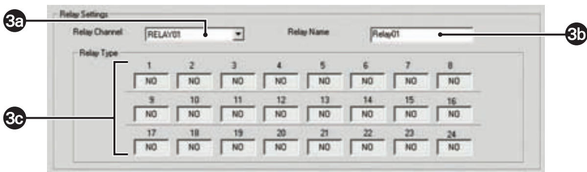
Figure 97. Relay and Alarm Settings Page: Relay Settings Section
