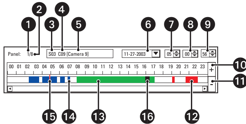
Figure 53. Playback Timeline
