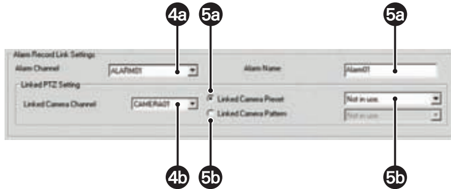
Figure 108. Event-PTZ Link Settings: Linking Presets and Patterns to Alarm Events
