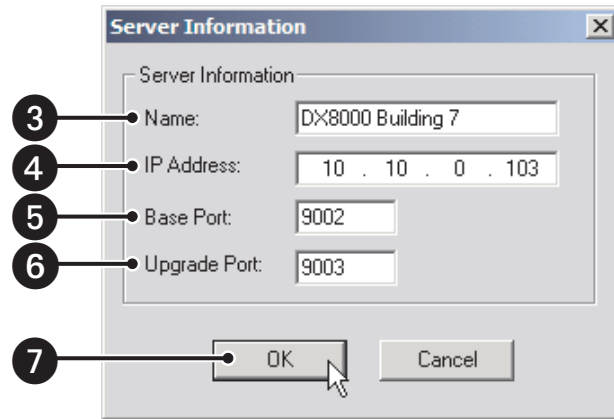
Figure 13. Server Information Dialog Box
