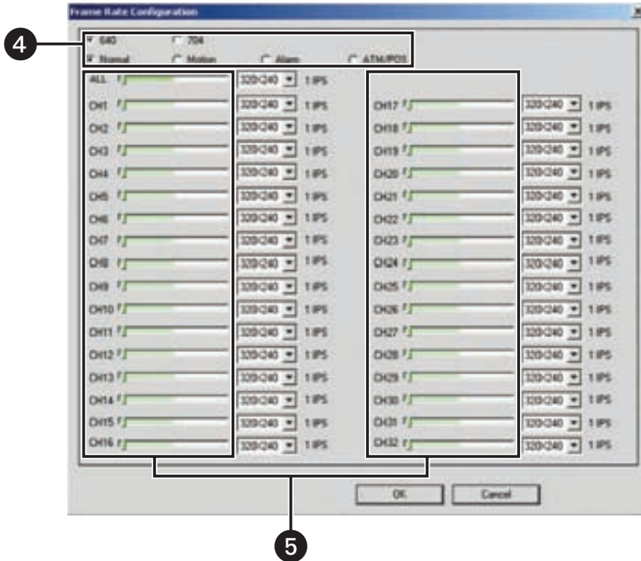
Figure 124. Frame Rate Configuration Dialog Box
