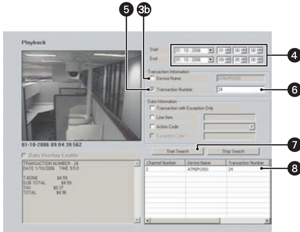
Figure 66. Searching an POS Event by Transaction Number
