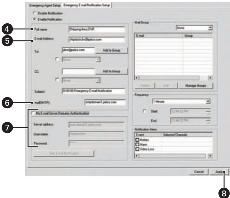
Figure 145. Basic E-mail Notification Setup
