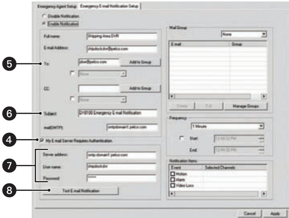
Figure 146. E-Mail Test
