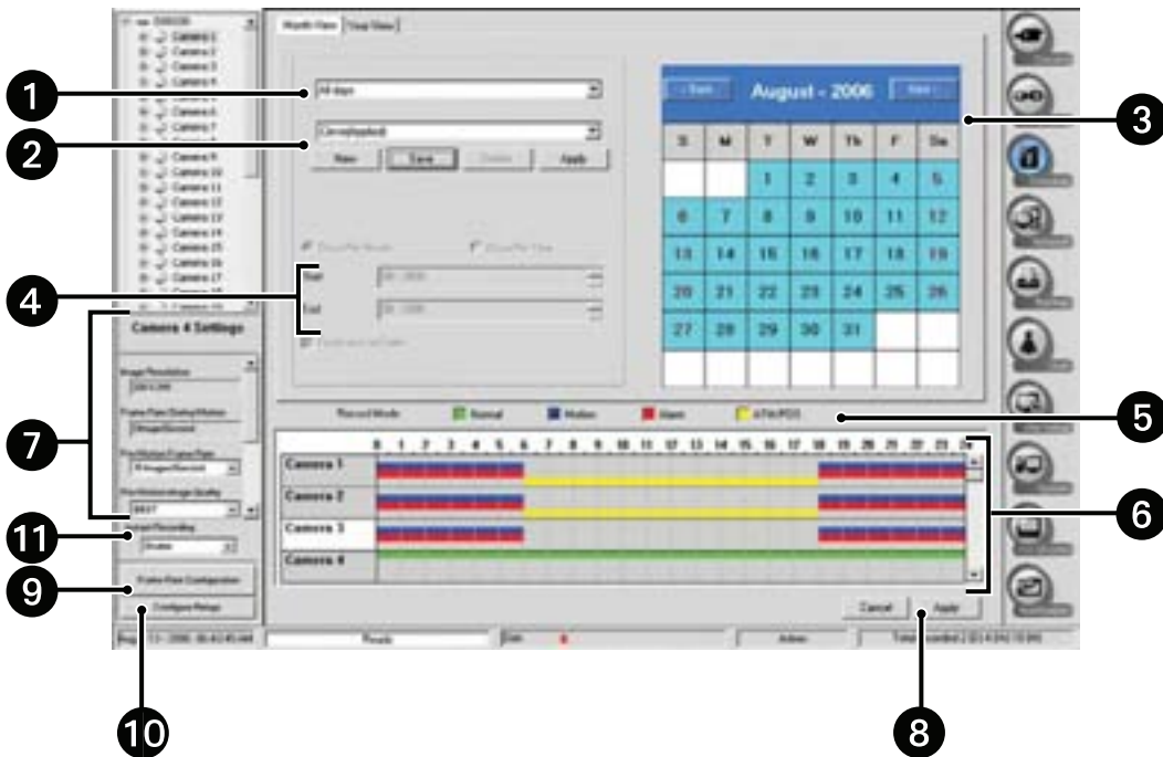
Figure 111. Schedule Page
