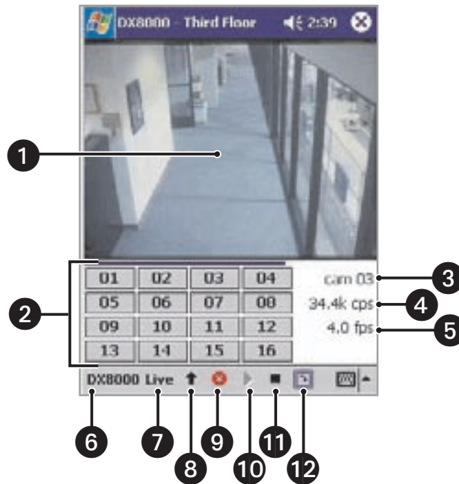
Figure 186. Main Screen
