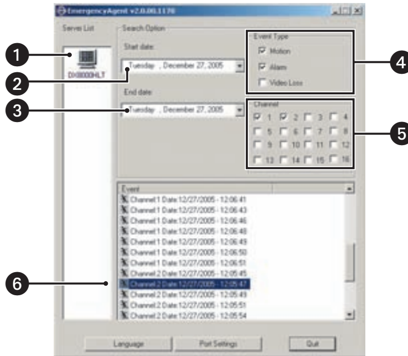
Figure 164. Client Emergency Agent Server List and Log
