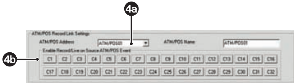
Figure 105. Event-Recording Link Settings: ATM/POS Record Link Settings Section
