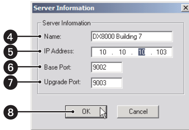
Figure 15. Editing Server Information
