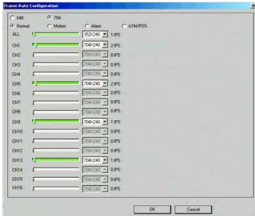
Figure 127. Frame Rate Configuration Screen
