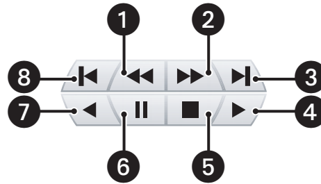
Figure 51. Playback Controls
