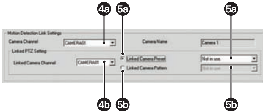
Figure 107. Event-PTZ Link Settings: Linking Presets and Patterns to Motion Events
