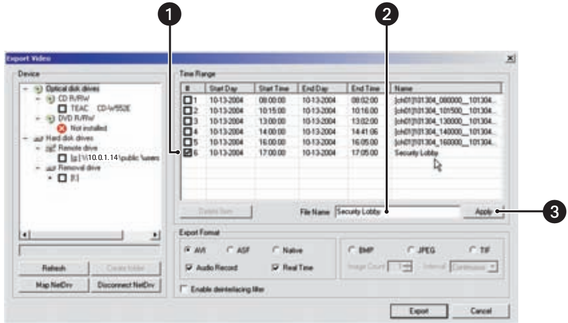
Figure 85. Renaming Export Time Ranges
