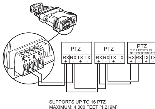
Figure 5. PTZ Installation
