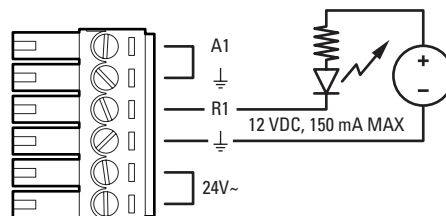
Figure 9. Relay Wiring
