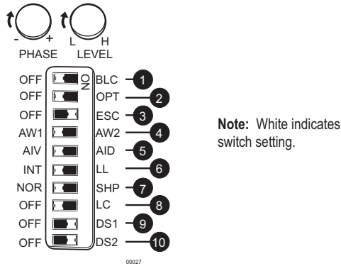
Figure 6. DIP Switch Default Settings
