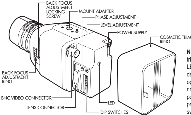
Figure 1. Camera Layout
