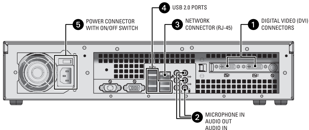
Figure 11. Rear Panel Connections
