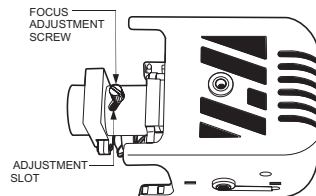
BOTTOM VIEW OF CAMERA WITH HEATER BOARD REMOVED
