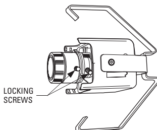
VARIFOCAL LENS
