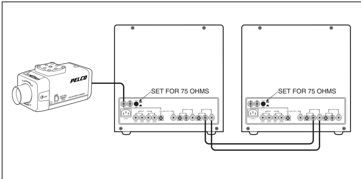
Figure 6. Output Connections
