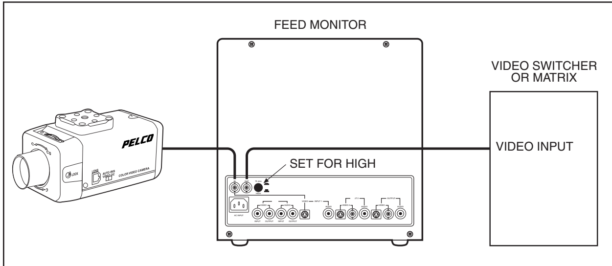
Figure 5. Dedicated Monitor Application with No Control
