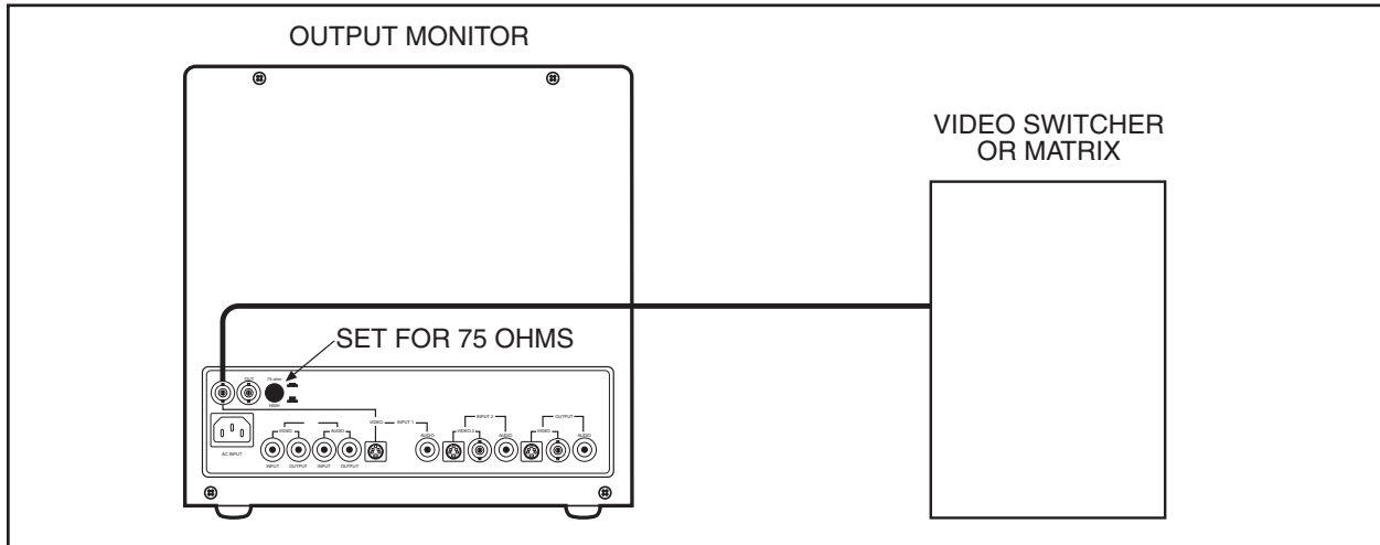
Figure 3. Input from Switcher or Matrix Control System
