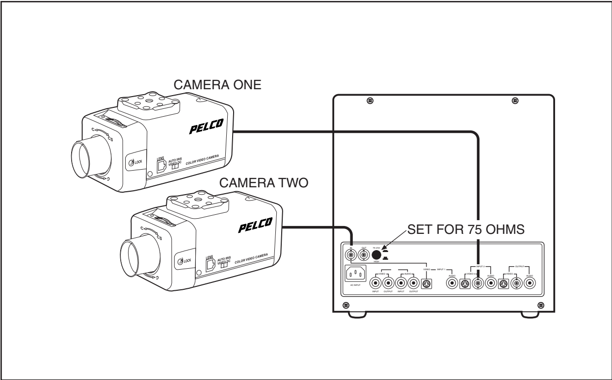
Figure 2. Camera Inputs
