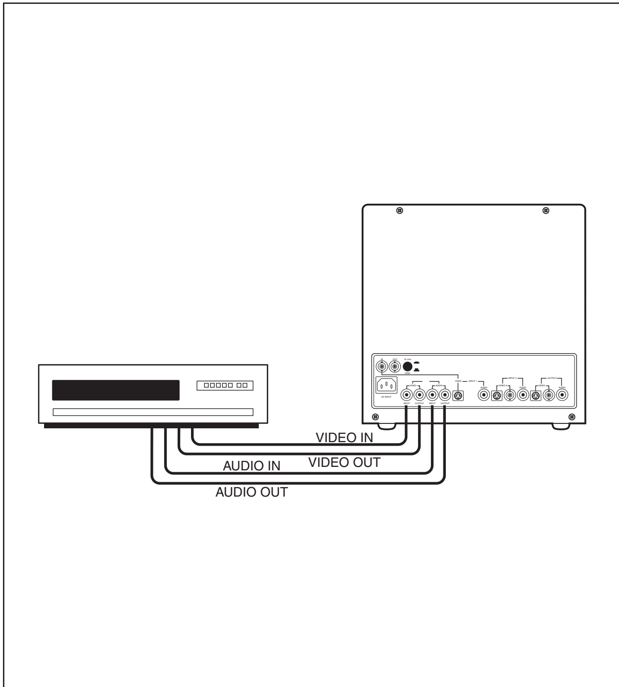
Figure 7. VTR Connections
