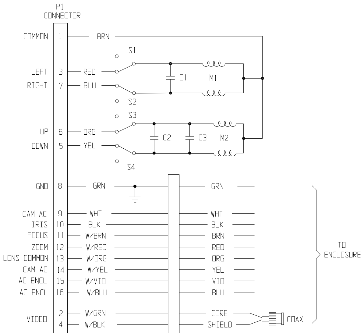
Figure 3. PT1280P/PT1280SL Wiring Diagram
