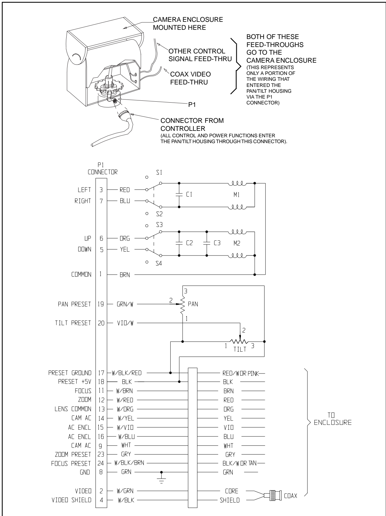
Figure 5. PT1280P/PP Wiring Diagram
