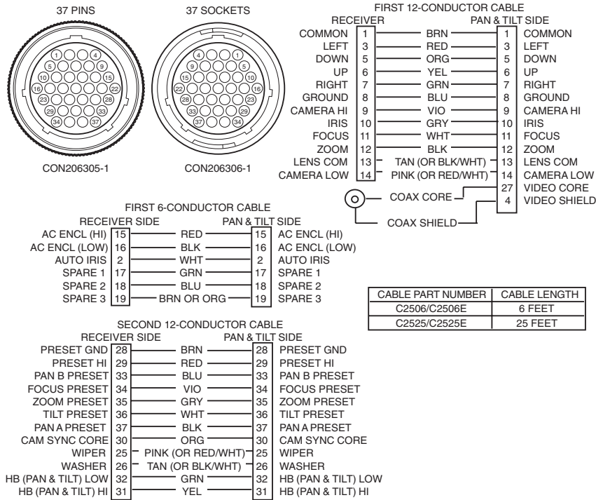
Figure 1. Wiring Diagram
