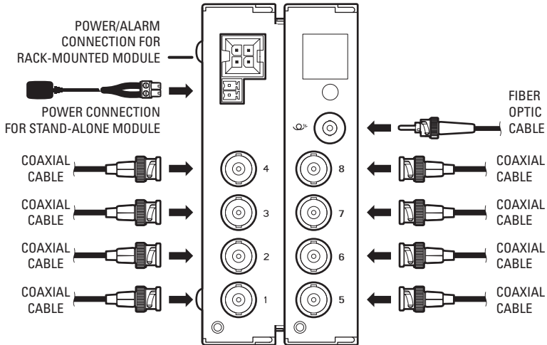
Figure 7. FT8308 Transmitter/FR8308 Receiver Connections
