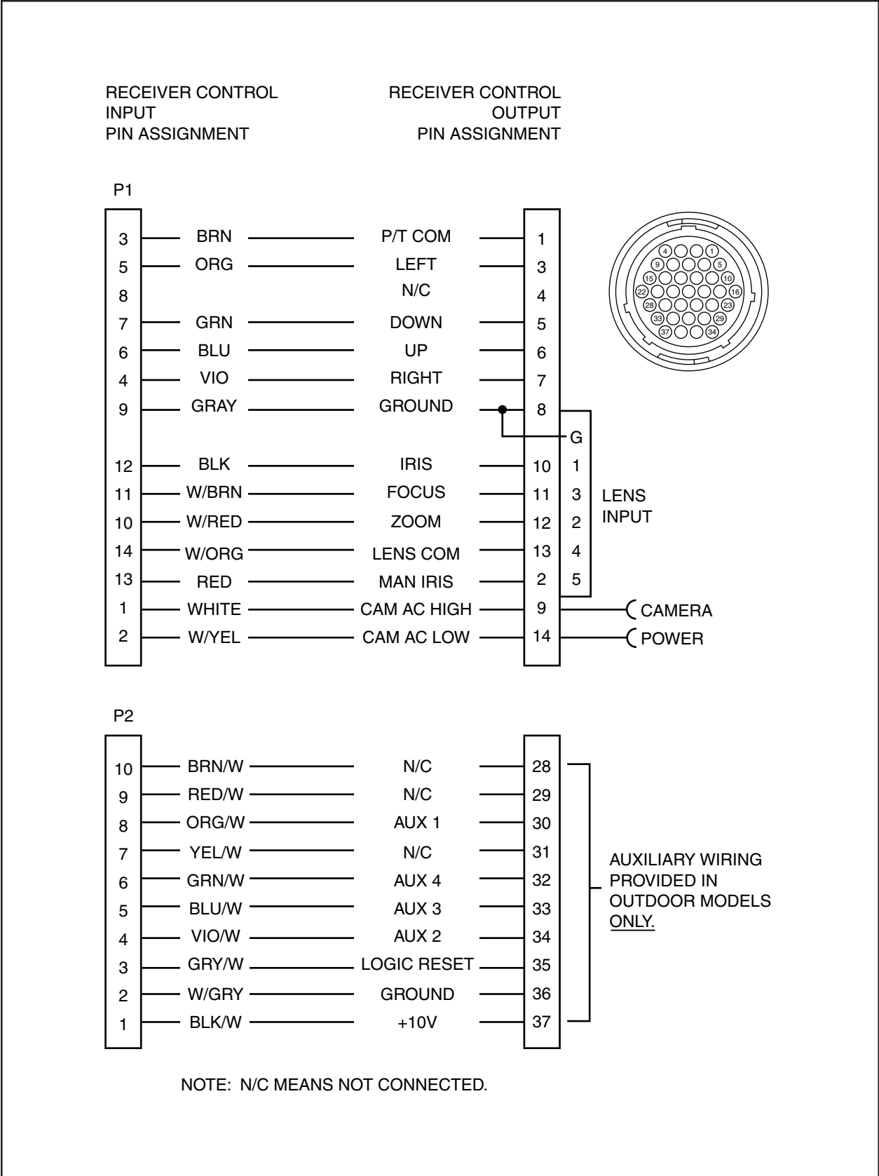
Figure 7. Receiver Control Output/Input Pin Assignments
