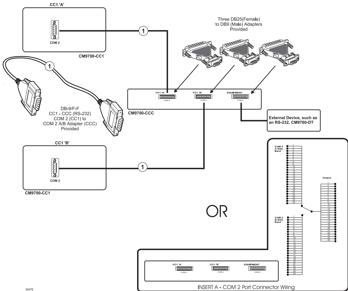
Figure 1-6. COM 2 Port Options
