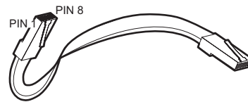
Figure 1-9. RJ-45 Pin Detail
