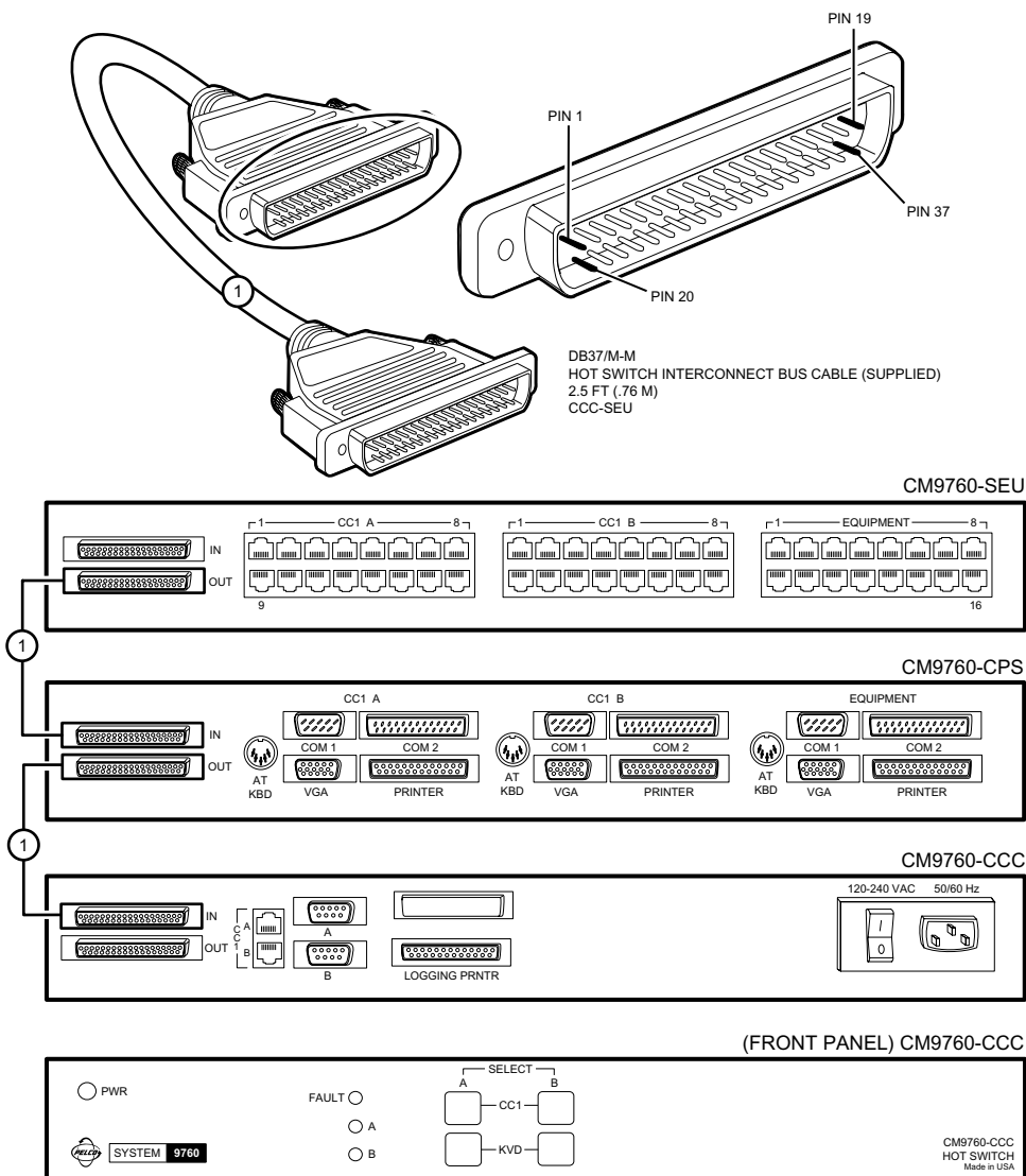
Figure 1-3. HS Rear Views and CCC Subunit Front Panel
