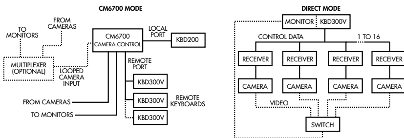
Figure 1. KBD300V Applications
