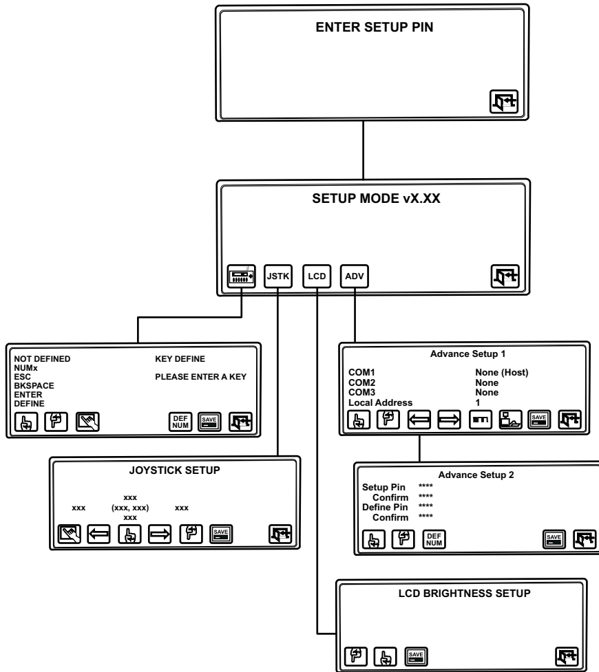
Figure 45. Setup Mode Menu Tree (DIP Switch 2 ON)
