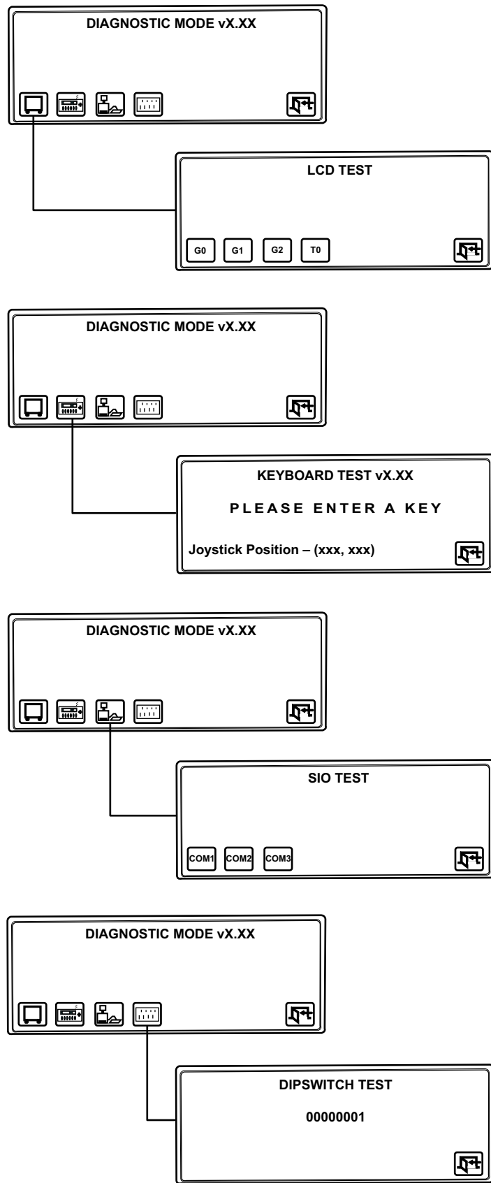
Figure 46. Diagnostic Mode Menu Tree (DIP Switch 1 ON)
