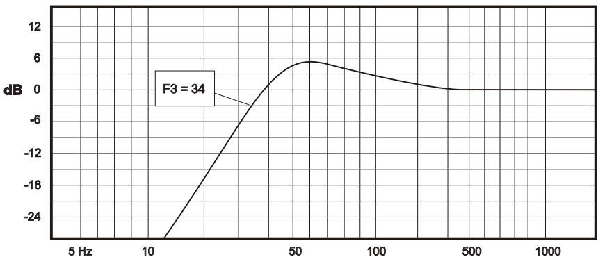
QC15S4 AMPLITUDE RESPONSE (DB/HZ)
