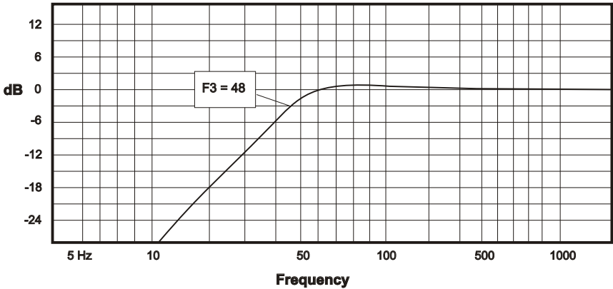
QC15S4 Amplitude Response (dB/Hz)
