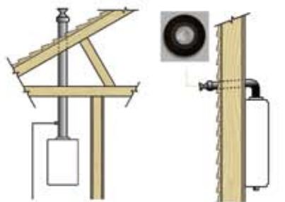
INTERIOR ROOF OR WALL VENTING The Rinnai can be vented vertically or horizontally.
