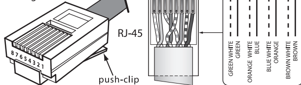
RJ-45 Using T568A Wiring Standard
