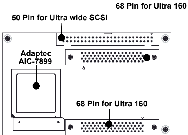
Figure 1.3: SCSI daughter board
