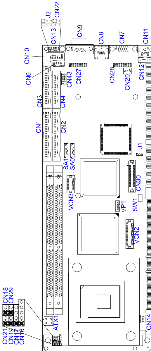
Figure 1.1: Jumper and Connector locations
