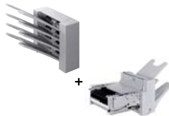
Combination: 4-Bin Mailbox (MBT-40S) and 2-Bin Finisher (SCX-FIN20S) Output capacity: 1000 sheets
