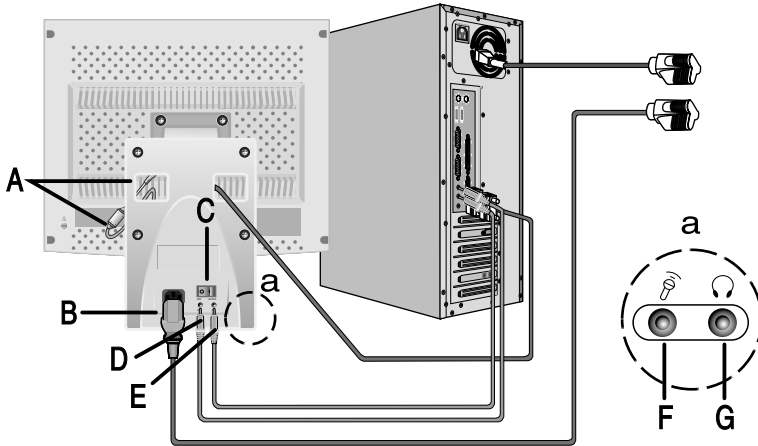
Figure 4. Multimedia connections
