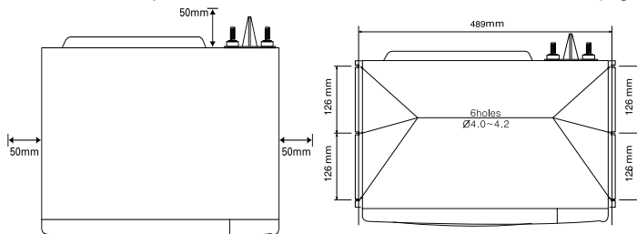
Front of Microwave Oven (Fig. 2)
