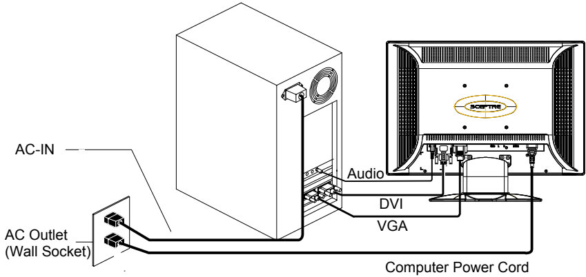
Figure 1-5: PC conenction
