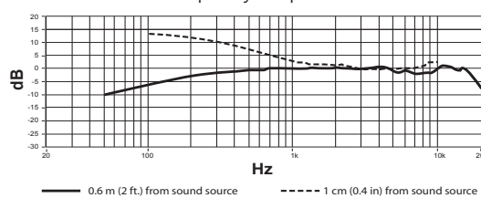
Frequency Response
