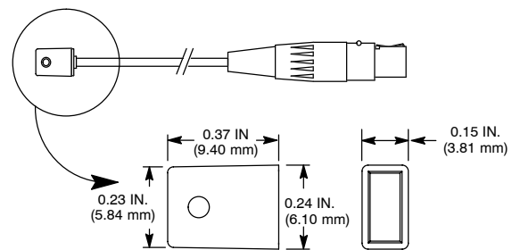
SM93/WL93 MICROPHONE
