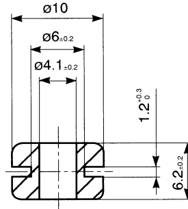
Fig. 7-1 Recommended Rubber foot
