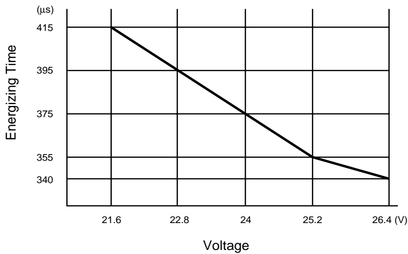
Fig. 3-10 Head Energizing Time - Head Power Supply Voltage
