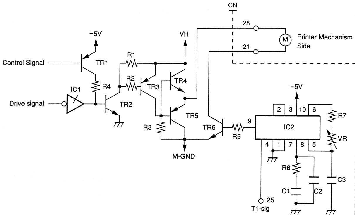
Fig. 3-15 Motor drive circuit (example)
