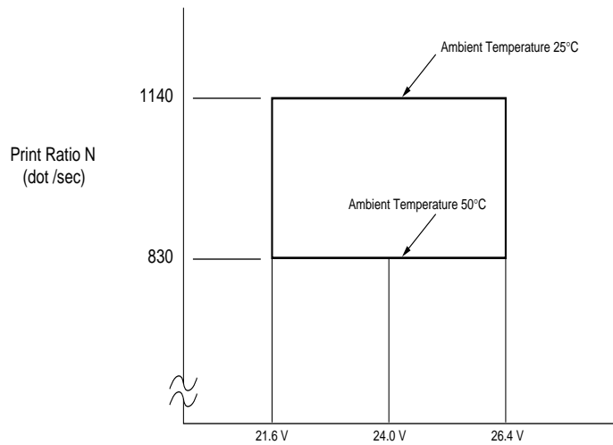
Fig. 3-12 Print duty
