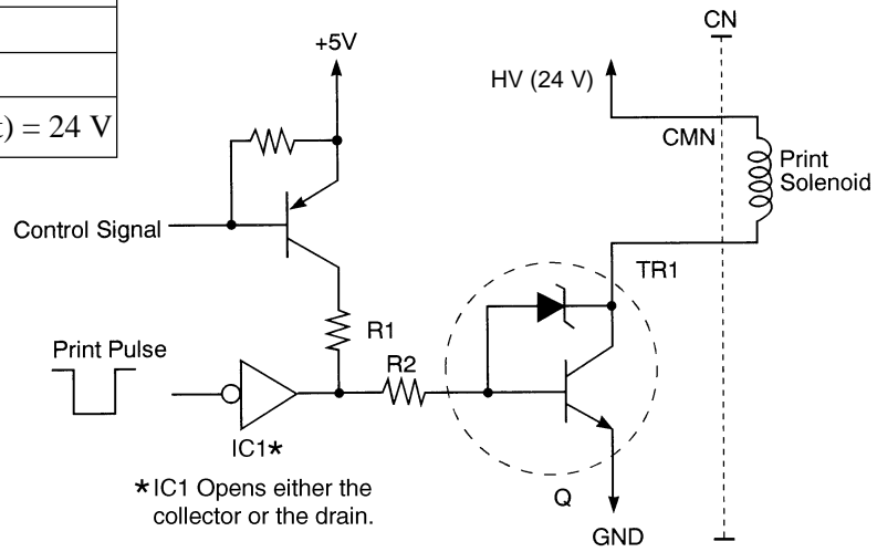
Fig. 3-11 Example of Print Solenoid Drive Circuit
