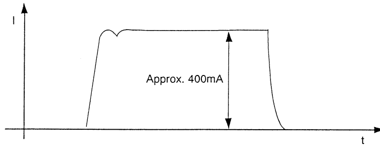
Fig. 3-17 Current waveform of RS-SOL
