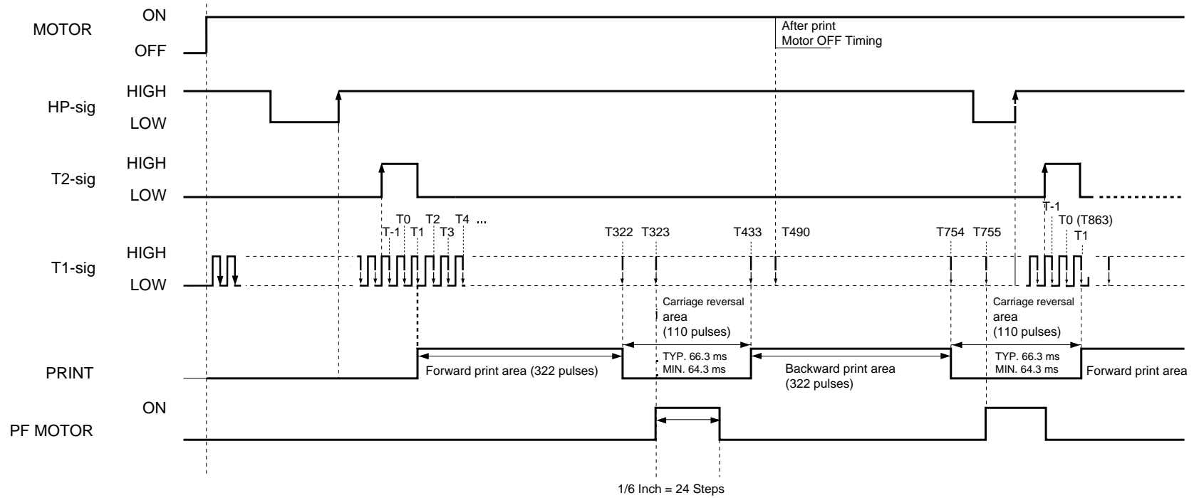
Fig. 3-7 Printing action
