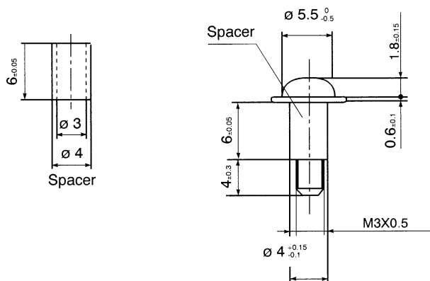
Fig. 7-2 Recommended Set screw (unit: mm)
