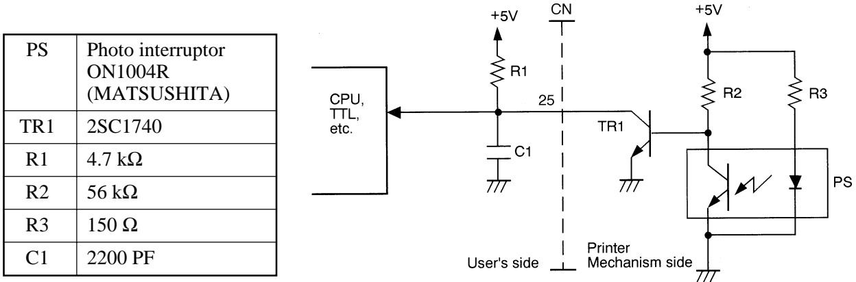
Fig. 3-19 Circuit of timing signal 1 (example)
