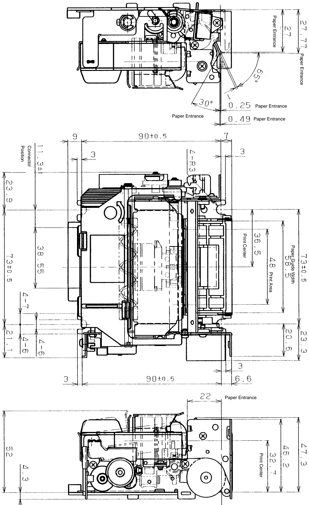
Figure 3-25 MP115MP External dimension (unit: mm)
