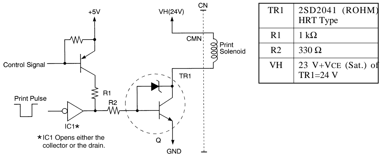
Fig. 8-3 Circuit to control drive circuit (example)
