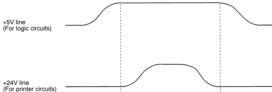
Fig. 8-1 Power supply ON/OFF timing rule
