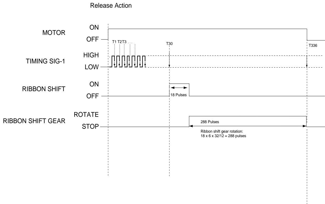
Fig. 3-8 Release action
