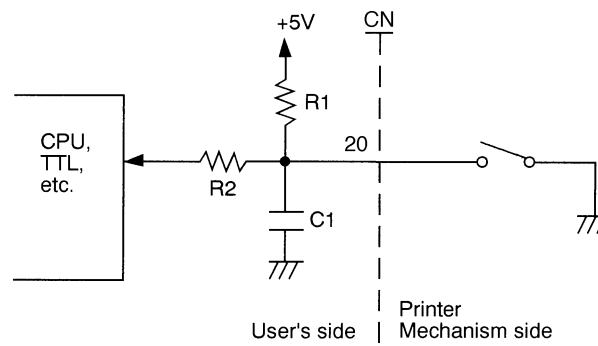
Fig. 3-22 Paper-out detector circuit (example)
