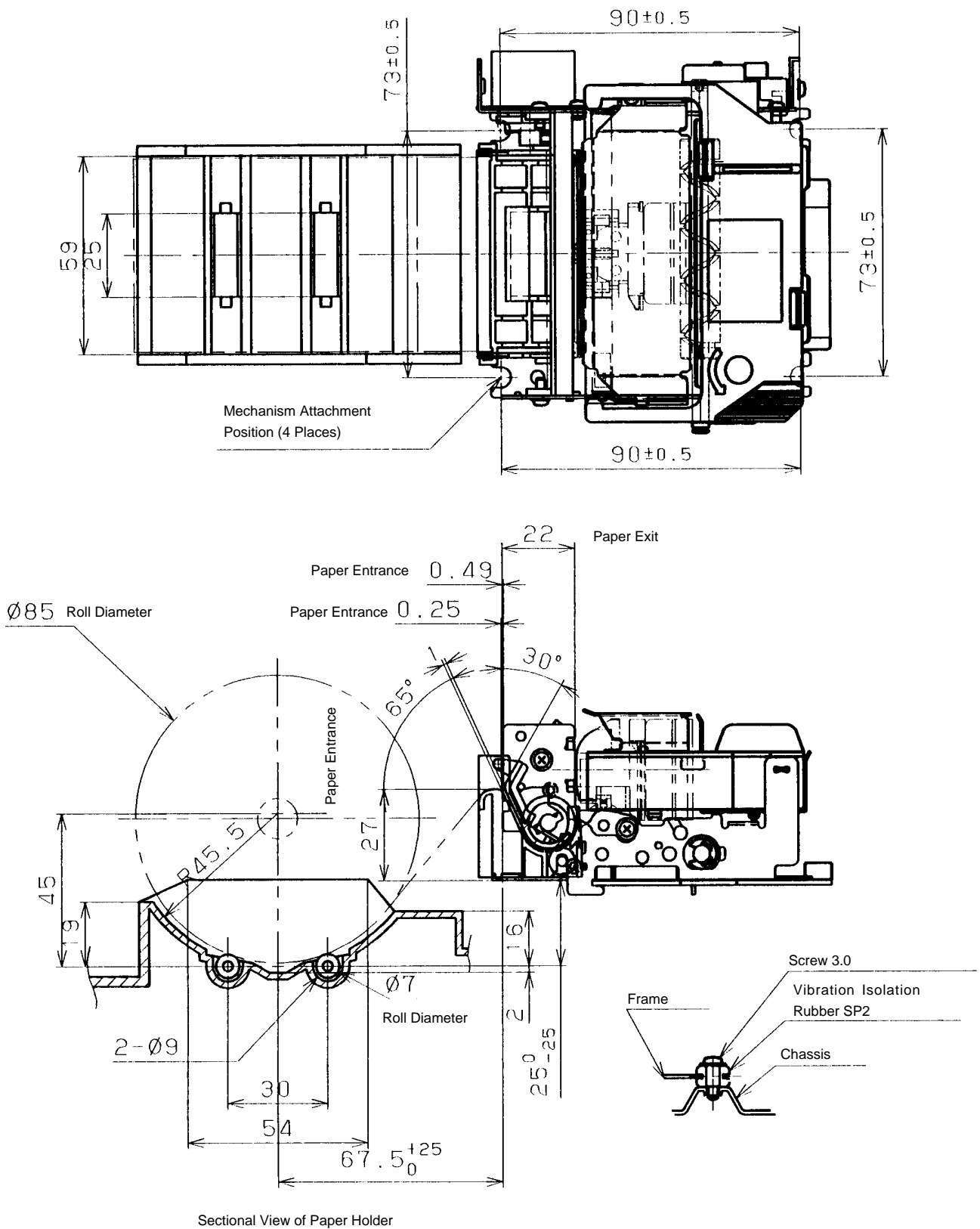
Fig. 7-4 Printer installation (example) (unit: mm)
