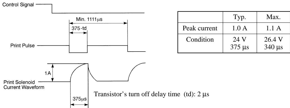
Fig. 3-9 Current waveform
