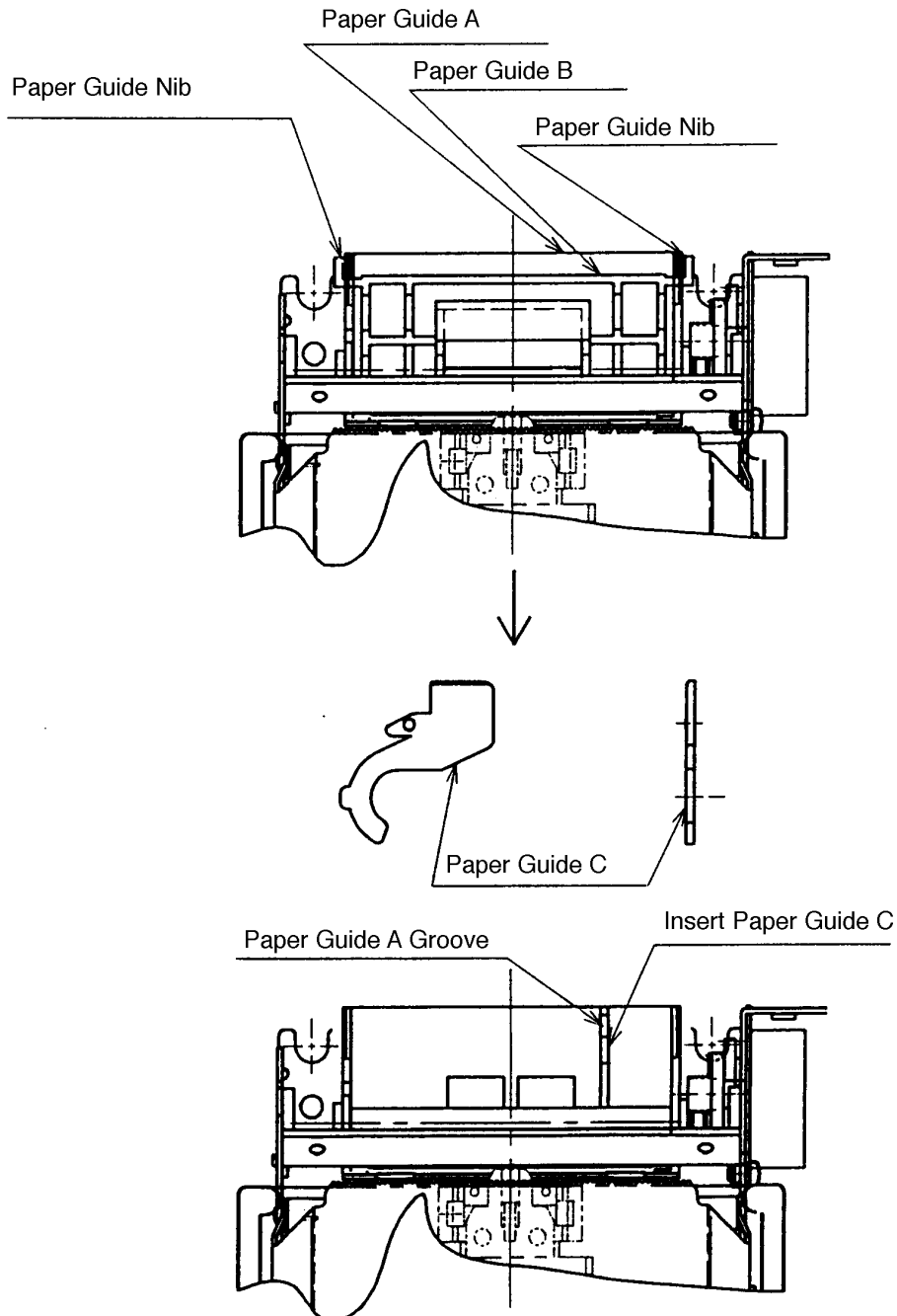
Fig. 10-1 Paper Guide Option
