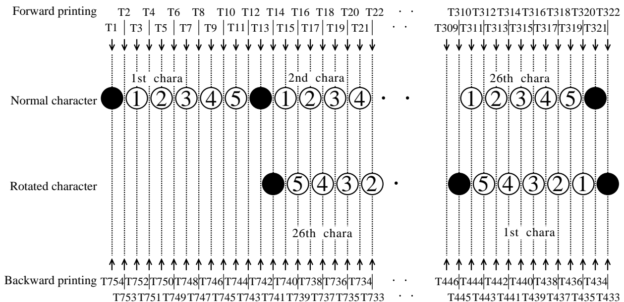
Fig. 3-6 Print Timing
