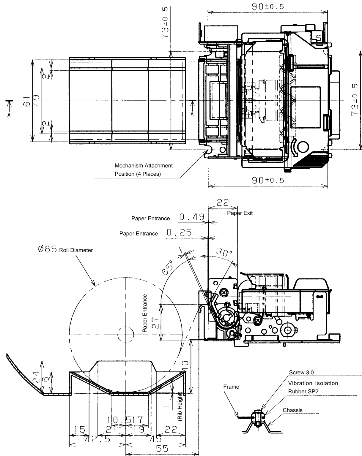
Sectional View of Paper Holder
