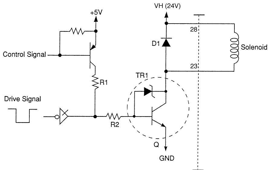
Fig. 3-18 RS-SOL drive circuit (example)
