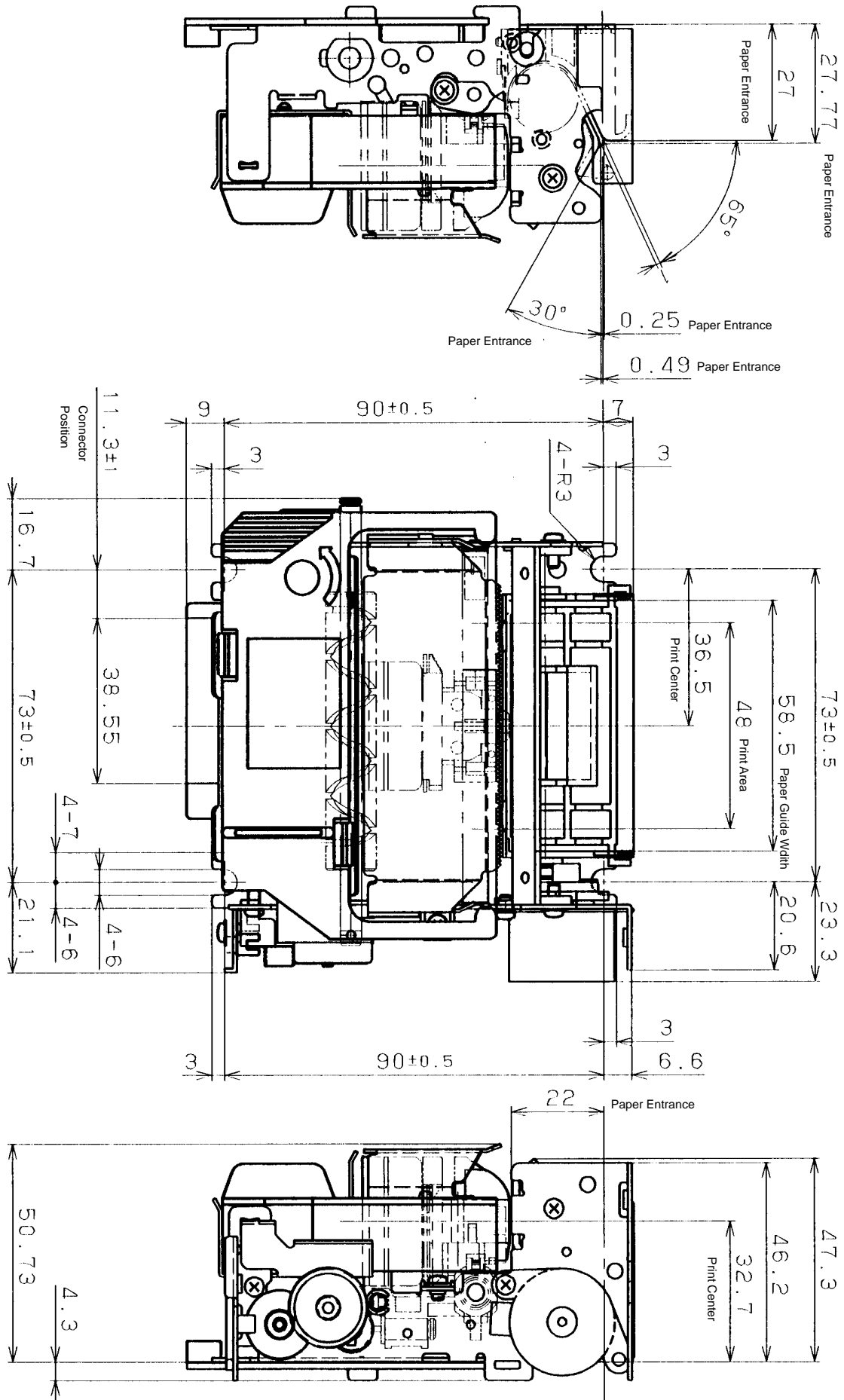
Figure 3-24 MP111MP External dimension (unit: mm)
