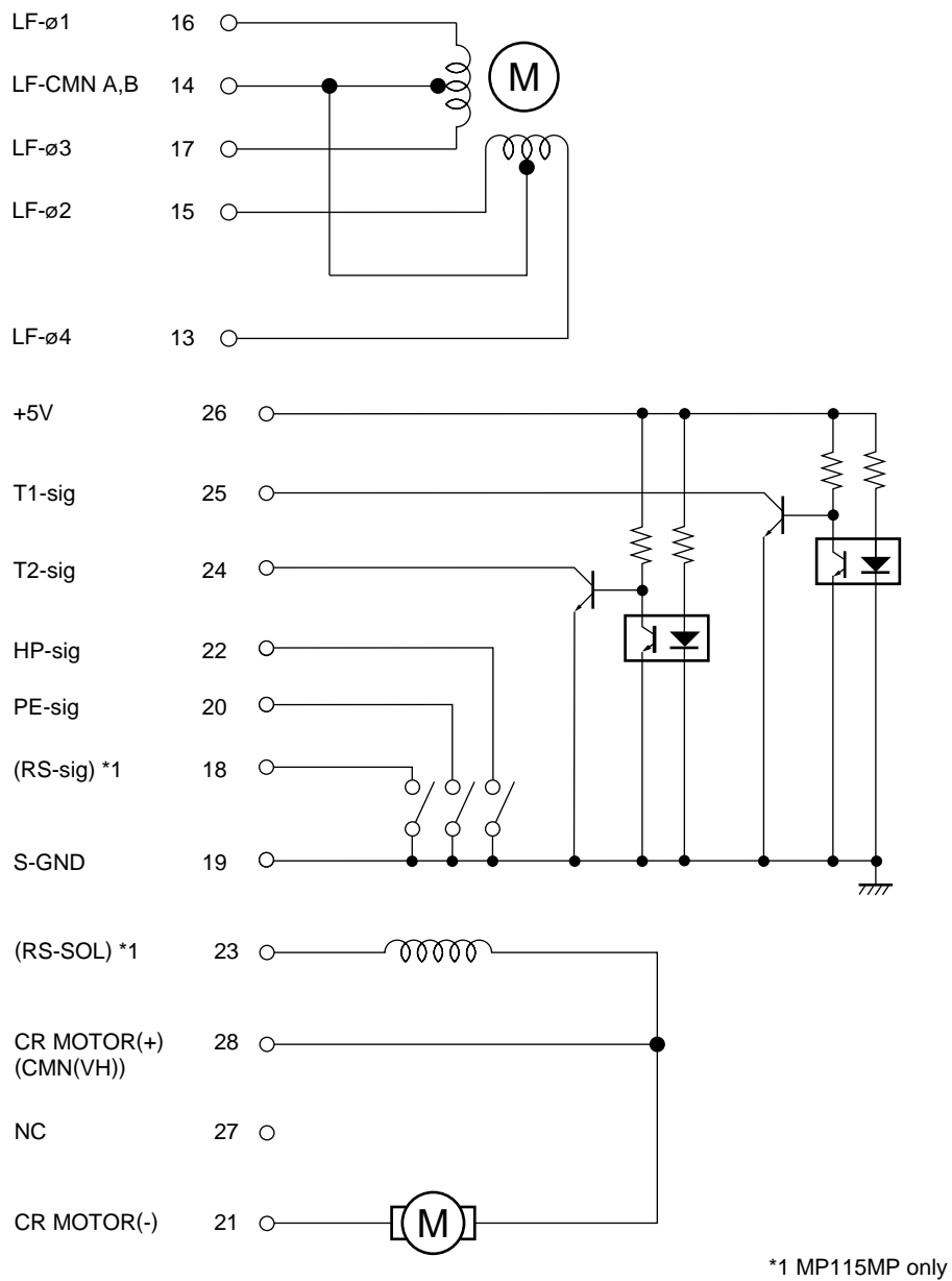
Fig. 3-5 Connector connections
