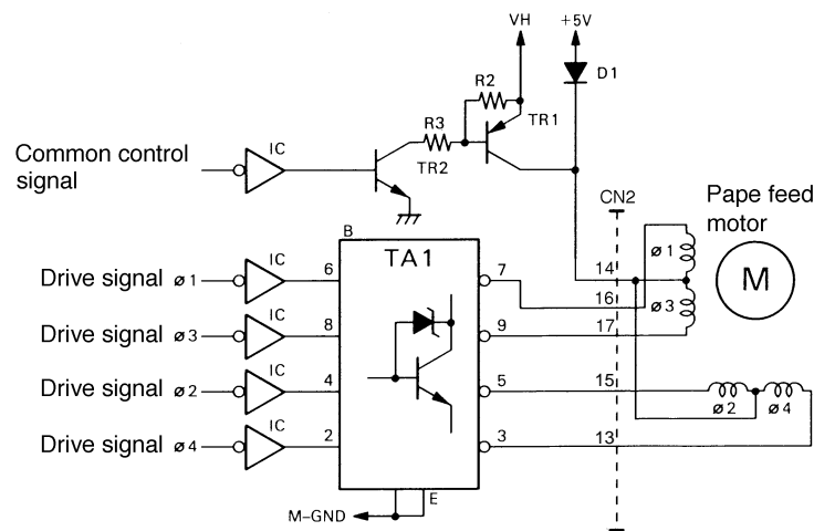
Fig. 3-16 Drive circuit of paper feed motor (example)
