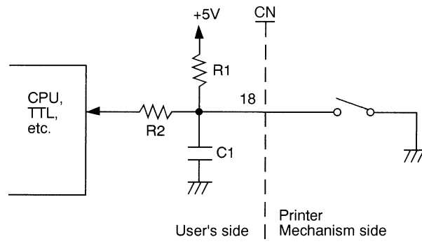
Fig. 3-23 Example of ribbon position detection circuit
