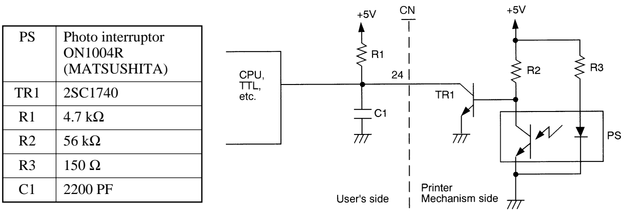
Fig. 3-20 Circuit of timing signal 2 (example)
