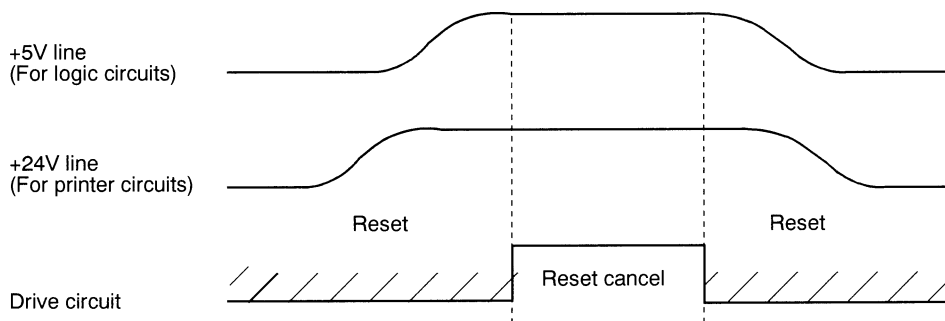
Fig. 8-2 Drive circuit controlling method
