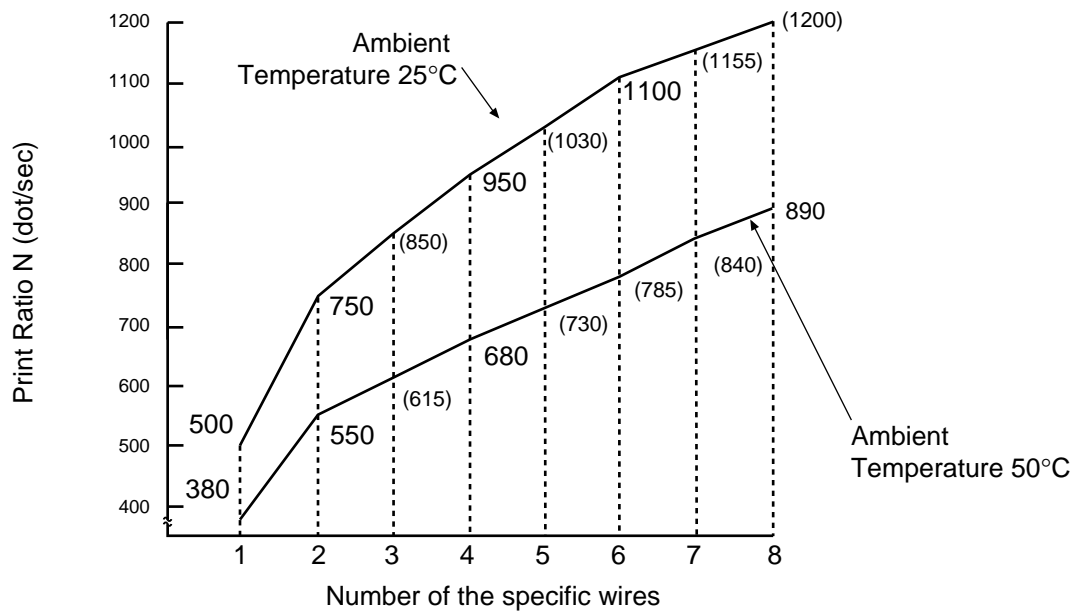
Fig. 3-13 Print duty (specific wires)
