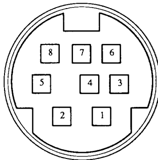
Interface Connector
