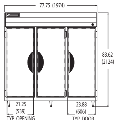
VSR-3 FRONT VIEW
