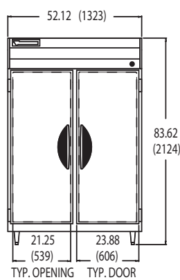
VSR-2 FRONT VIEW
