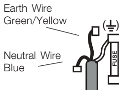
PLUG (with cover removed)
