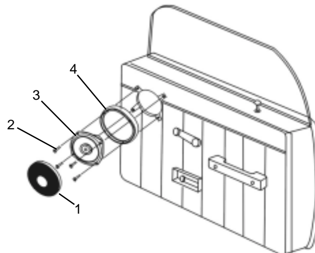
Securing Speaker and Grille
