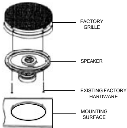
FACTORY SPEAKER REPLACEMENT
