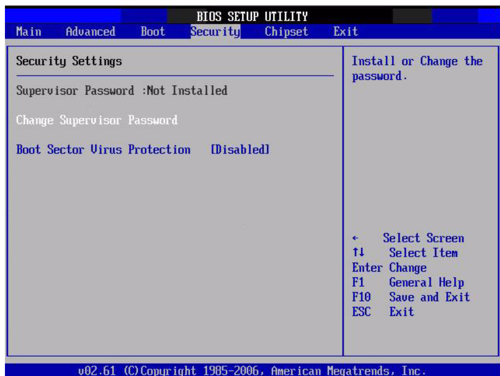
Figure 3.19 Password Configuration
