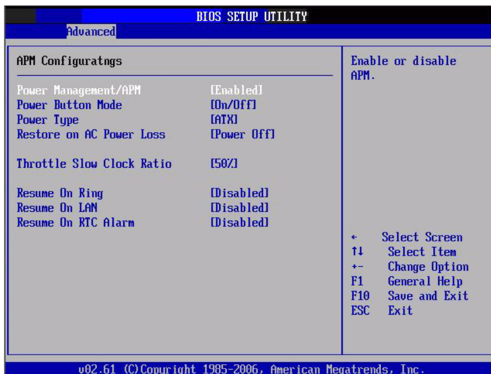
Figure 3.13 APM Configuration
