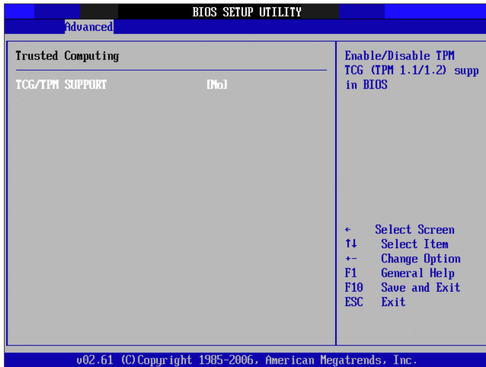
Figure 3.15 Trusted Computing
