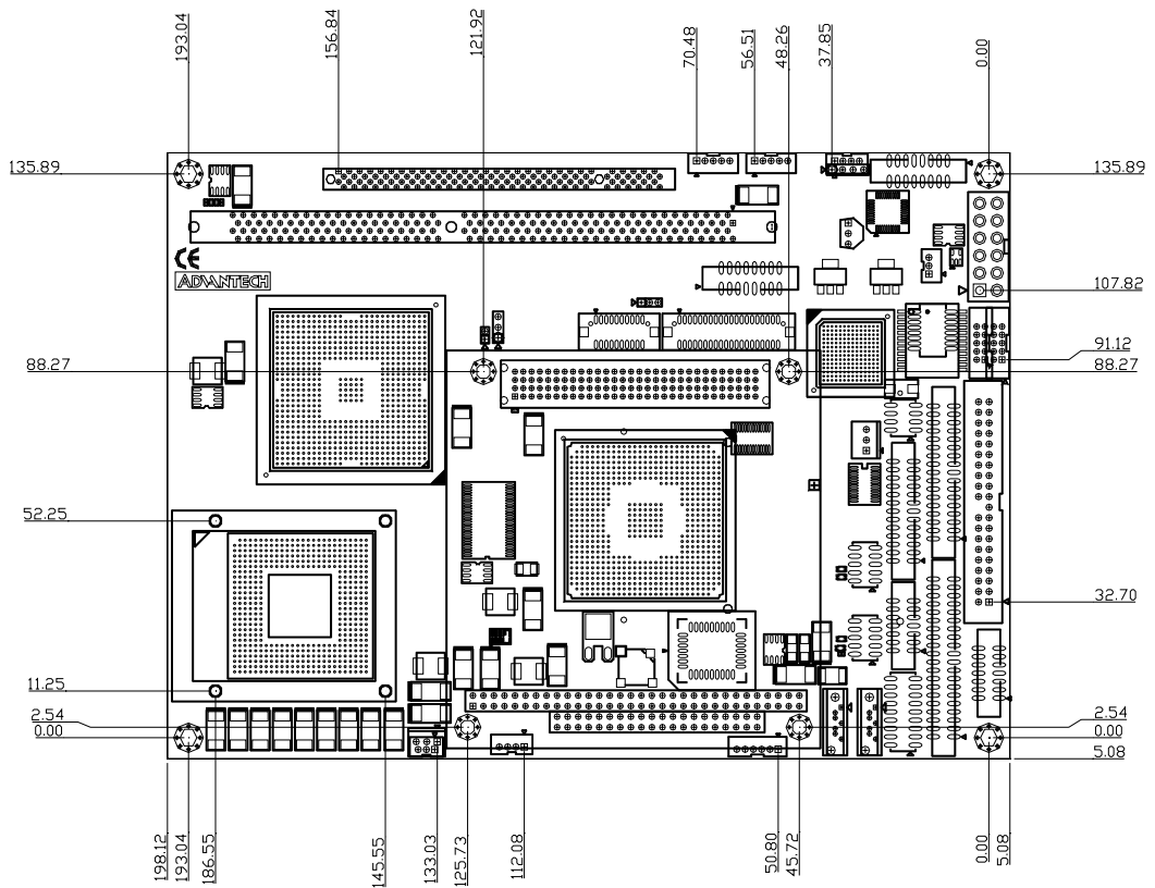
Figure E.1 PCM-9587 Mechanical Drawing (component side)
