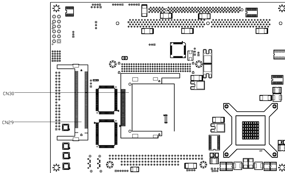
Figure 2.2 Jumper & Connector (solder side)
