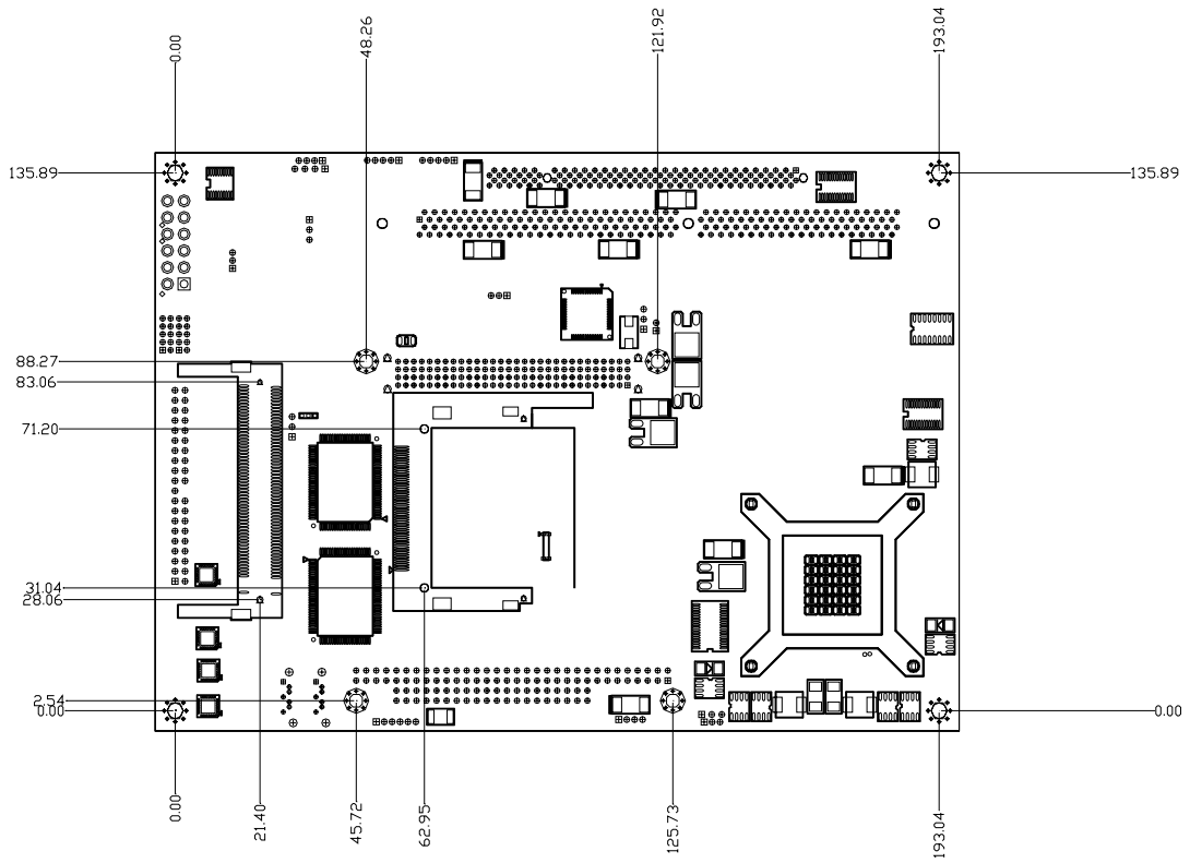
Figure E.2 PCM-9587 Mechanical Drawing (solder side)
