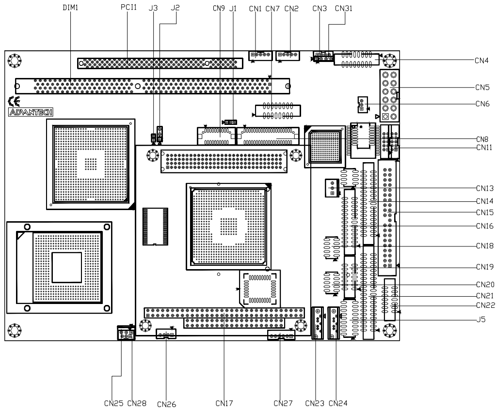
Figure 2.1 Jumper & Connector (component side)
