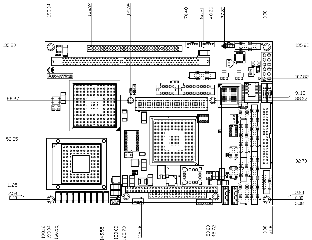
Figure 1.1 Board layout: dimensions (component side)
