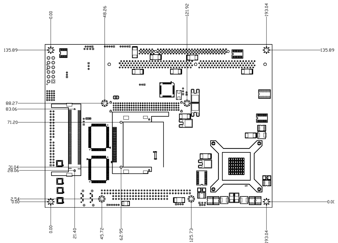
Figure 1.2 Board layout: dimensions (solder side)
