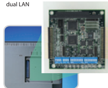
PCI-104 expansion
