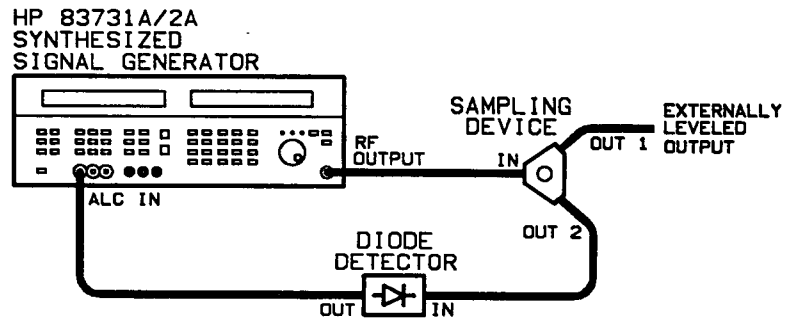
Figure 6-2. External Diode Detector Leveling Setup
